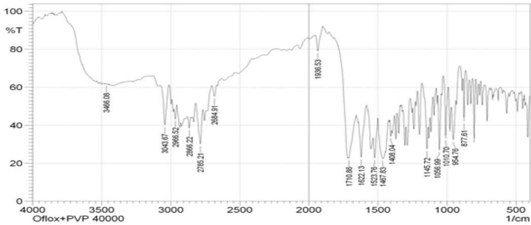
Figure 8: FT-IR Spectrum of Ofloxacin with PVP 40000
