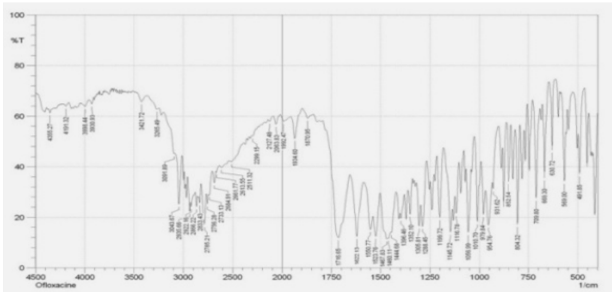
Figure 3: FT-IR Spectrum of Ofloxacin
